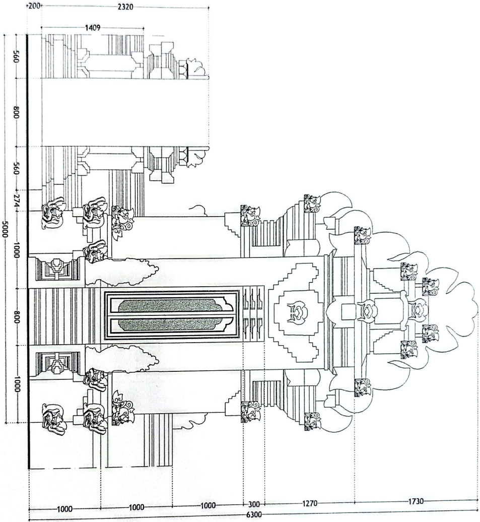
PURA SADA ARCHITECTURAL DRAWING TAMPAK DEPAN KORI AGUNG 1 : 30
