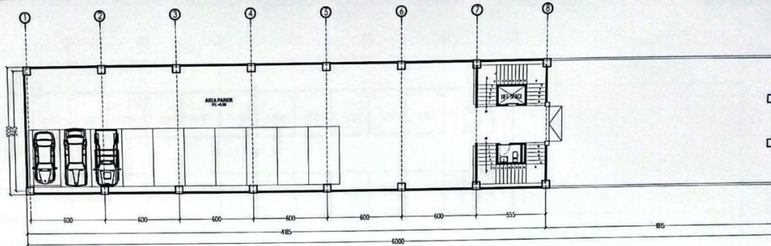
Scale 1:200 DENAH LANTAI 1
